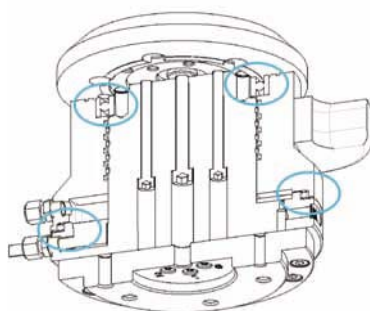
Rotary distributor with ball-bearing (marked in blue)
