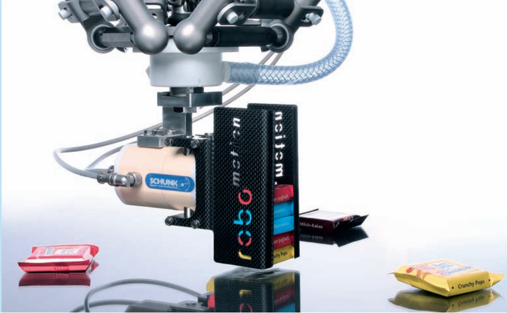
Workpieces stored within a stack gripper
