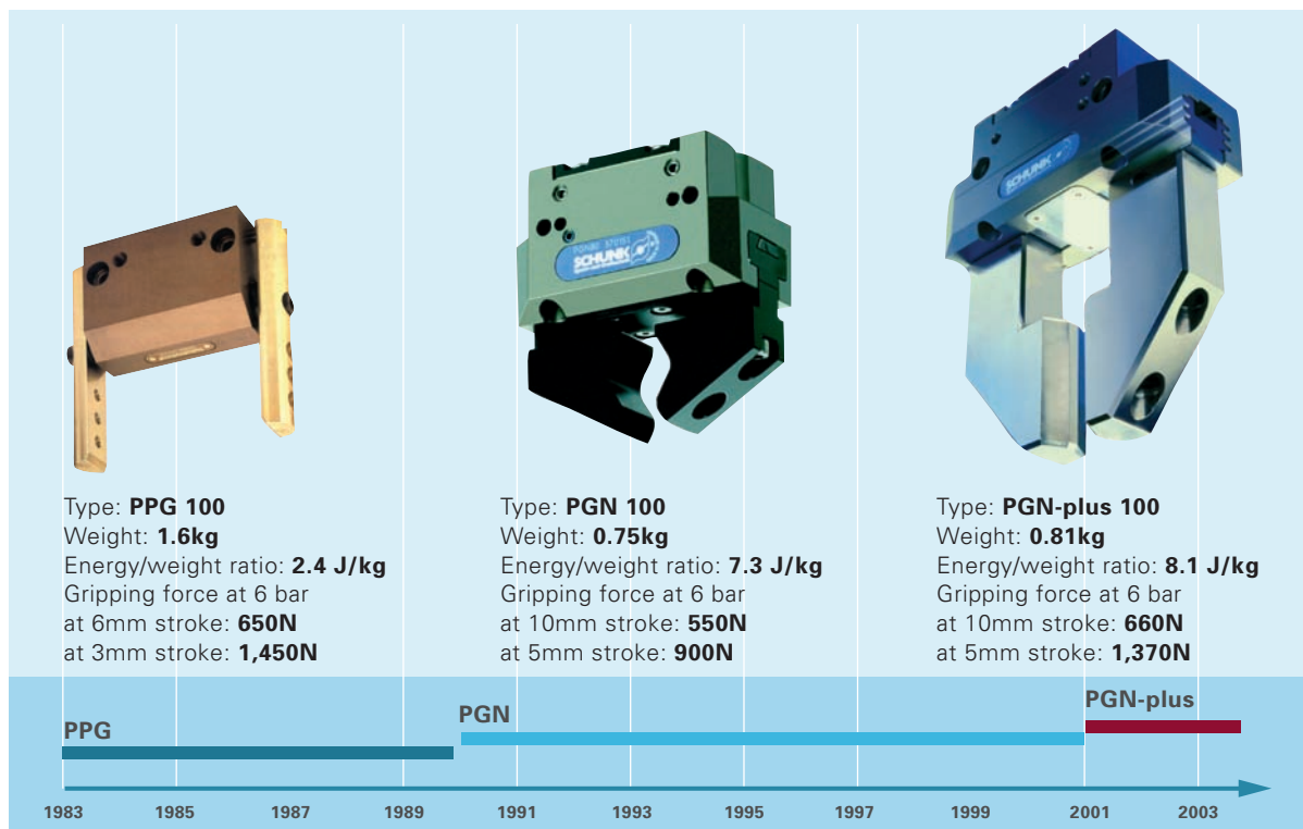
Figure 2.3 Comparing parallel grippers as an example for efficiency increase
