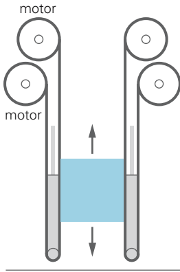
Figure 3.7 Flexible gripper finger – principle of function (source: SRI)
