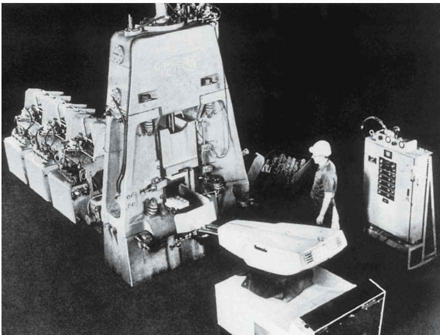
Unimate feeding a press (source: Fraunhofer IPA)
