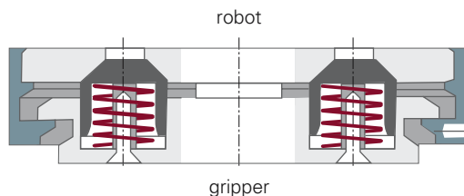
overload protection unit based on spring force
