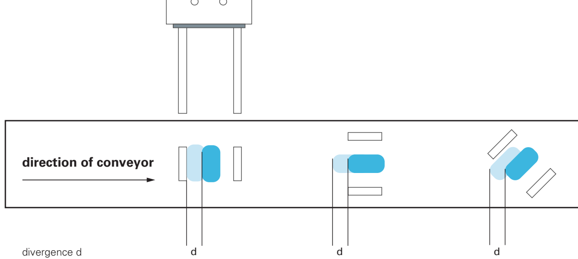
Figure 3.21 Workpiece divergence as a result of faulty synchronization during transport on conveyors
