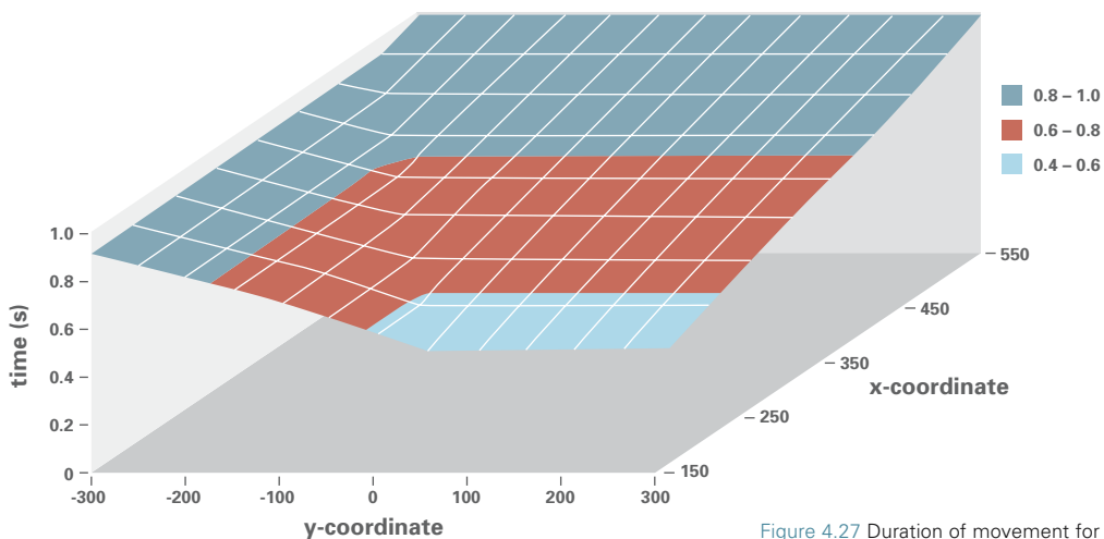
Figure 4.27 Duration of movement for a defined placing point of a linear gantry
