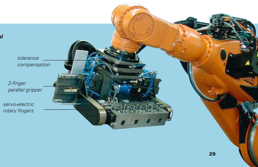
Figure 1.6 Example of a gripper system
