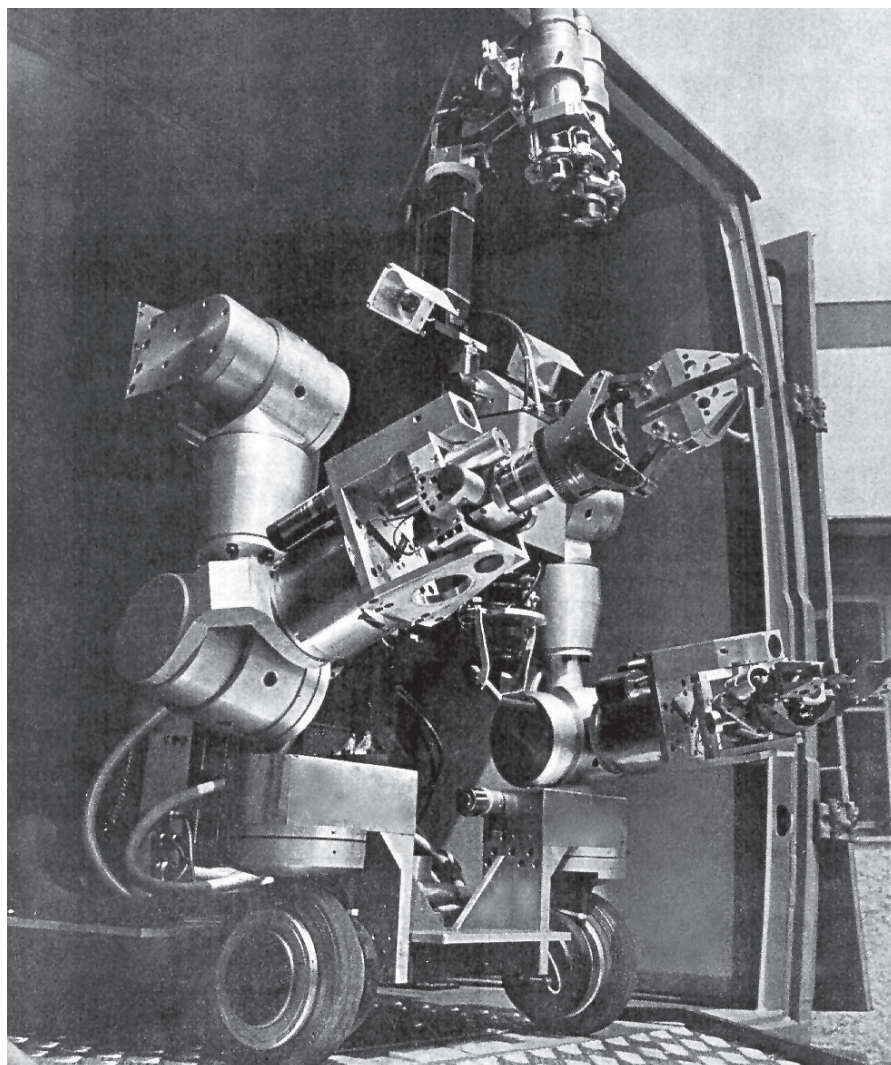
Syntelmann II Electric tele manipulator with 9 degrees of freedom per arm, position- and force-controlled, sensors for forces, sounds, temperatures (in front); operator with exo-skeleton transducer system, force feedback system, and stereo image transmission system (in the back). (Source: K. H. Dröge)
