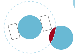
Figure 3.19 Interfering edges of workpieces in unsorted order status
