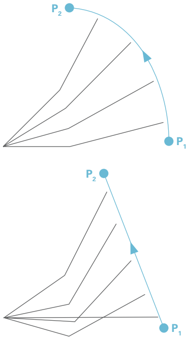
Figure 4.29 Movement under PTP control (above) and LIN path control (below)
