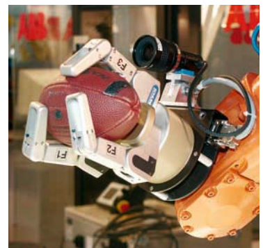
Barret Hand
