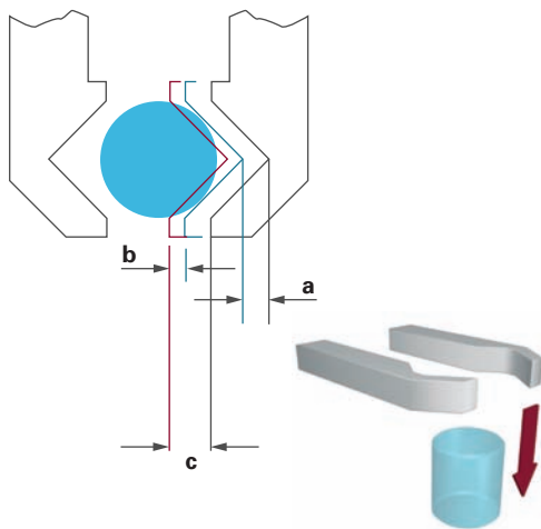
Figure 3.17 Axial grip
