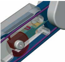
CAD image: sensors in the finger of the Barret Hand
