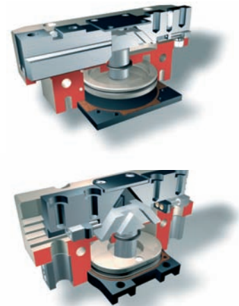
circular and elliptic piston surface
