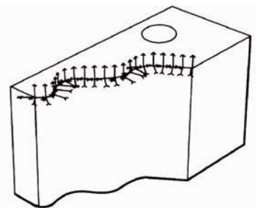
Robot path along a workpiece, generated from CAD data
