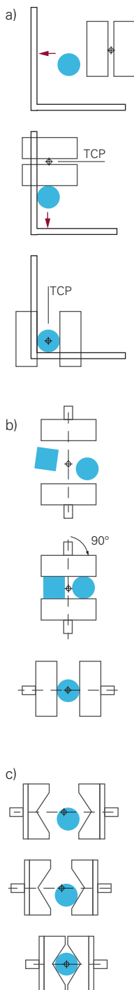
sliding grip a) external sliding grip b) internal sliding grip c) centering grip
