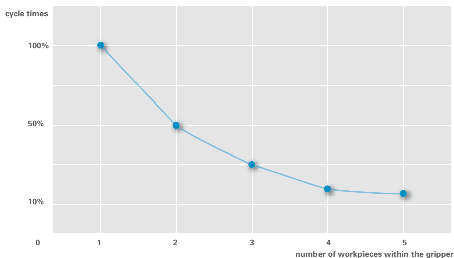
Figure 3.24 Efficiency increase by the principle of multiple gripping
