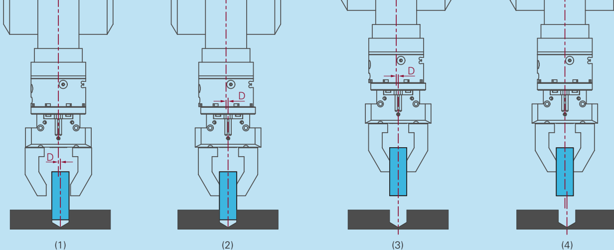
Figure 4.8 Principle of function: Compensation unit removing a bolt from its faulty position
