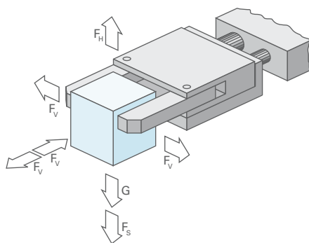
Figure 4.2 Dynamic gripping: forces of inertia must be compensated by translation
