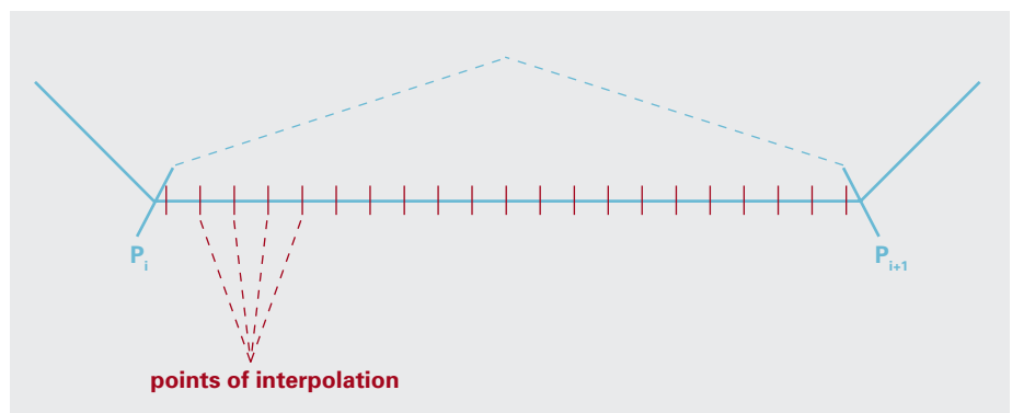
Figure 4.31 Section of a path with points of support and points of interpolation
