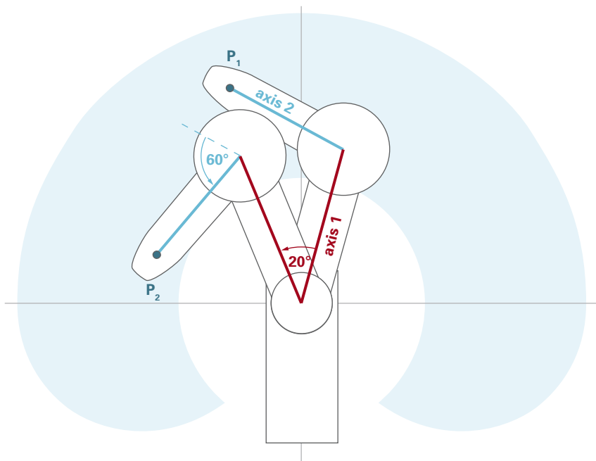
Figure 4.28 Robot movement subject to the condition that all axes are to reach their position as fast as possible
