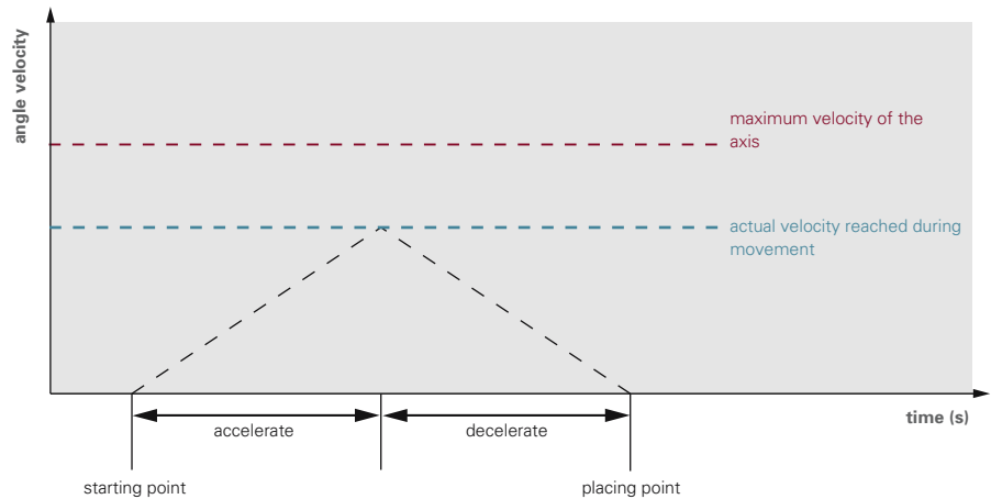
Figure 4.26 Velocity profile of a robot axis
