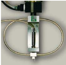
micro-components pick operation with adhesive grippers
