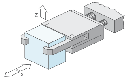
Figure 3.11 Form-fit gripping
