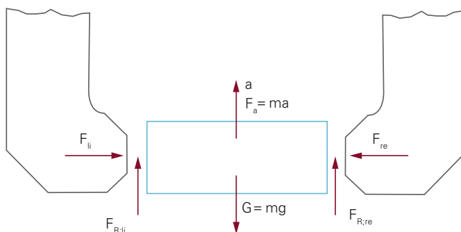
Figure 3.15 Decomposing forces on a workpiece for force-fit gripping
