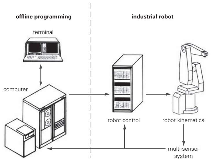
Figure 2.13 Offline programming in the early 80s
