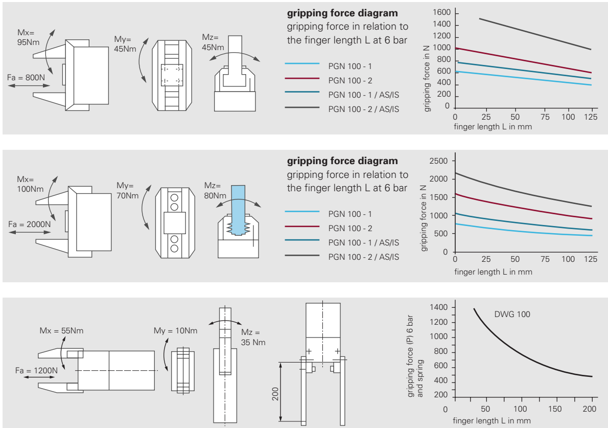
Figure 3.16 Different force distribution for various gripper types – maximum admissible forces and moments at the gripper fingers in addition to the gripping force.
