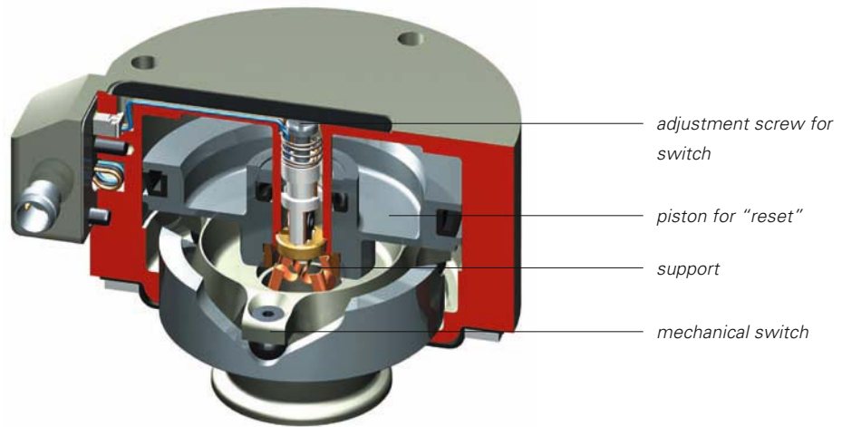
anti-collision unit, sectional view
