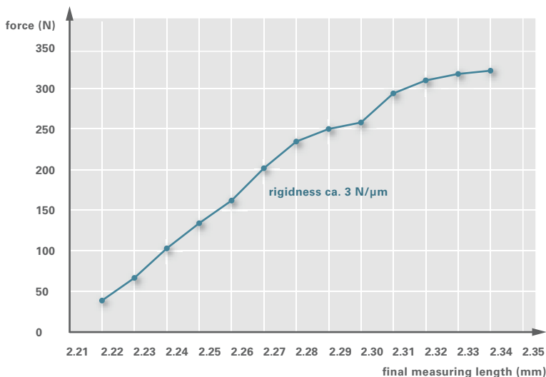
Figure 3.30 Dynamic gripping force measuring
