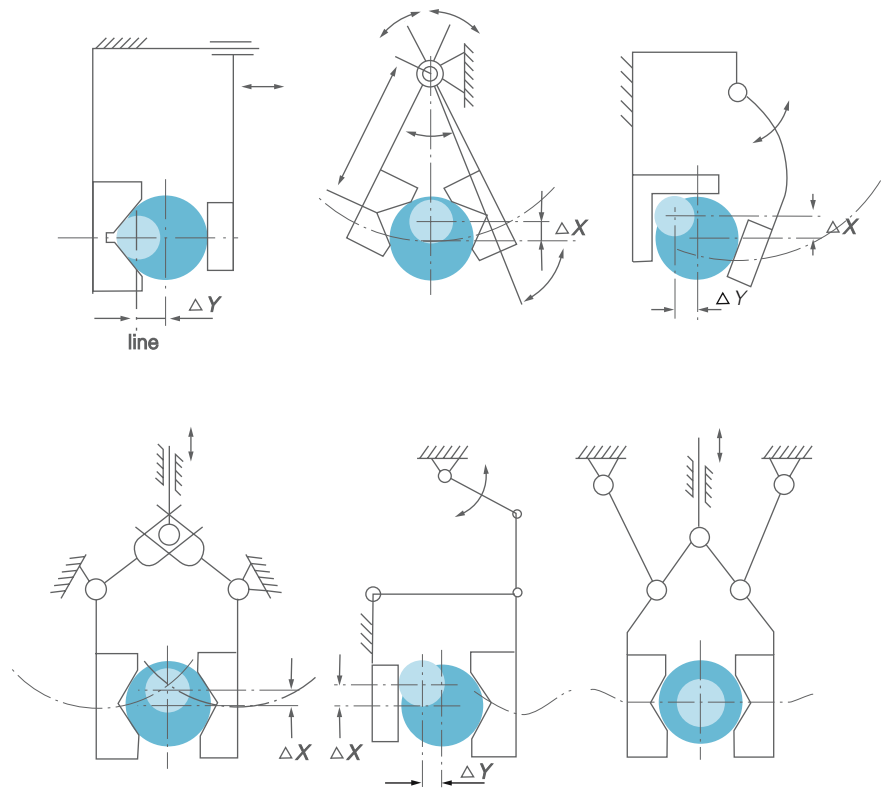
Figure 3.12 Movements of gripper fingers according to type of kinematics
