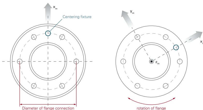
Figure 4.20 Flange plate according to DIN ISO 9409 and flange system of coordinates
