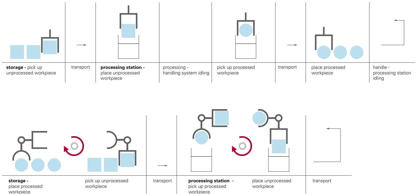
Figure 4.13 Feeding a processing machine without swivel unit and with swivel unit
