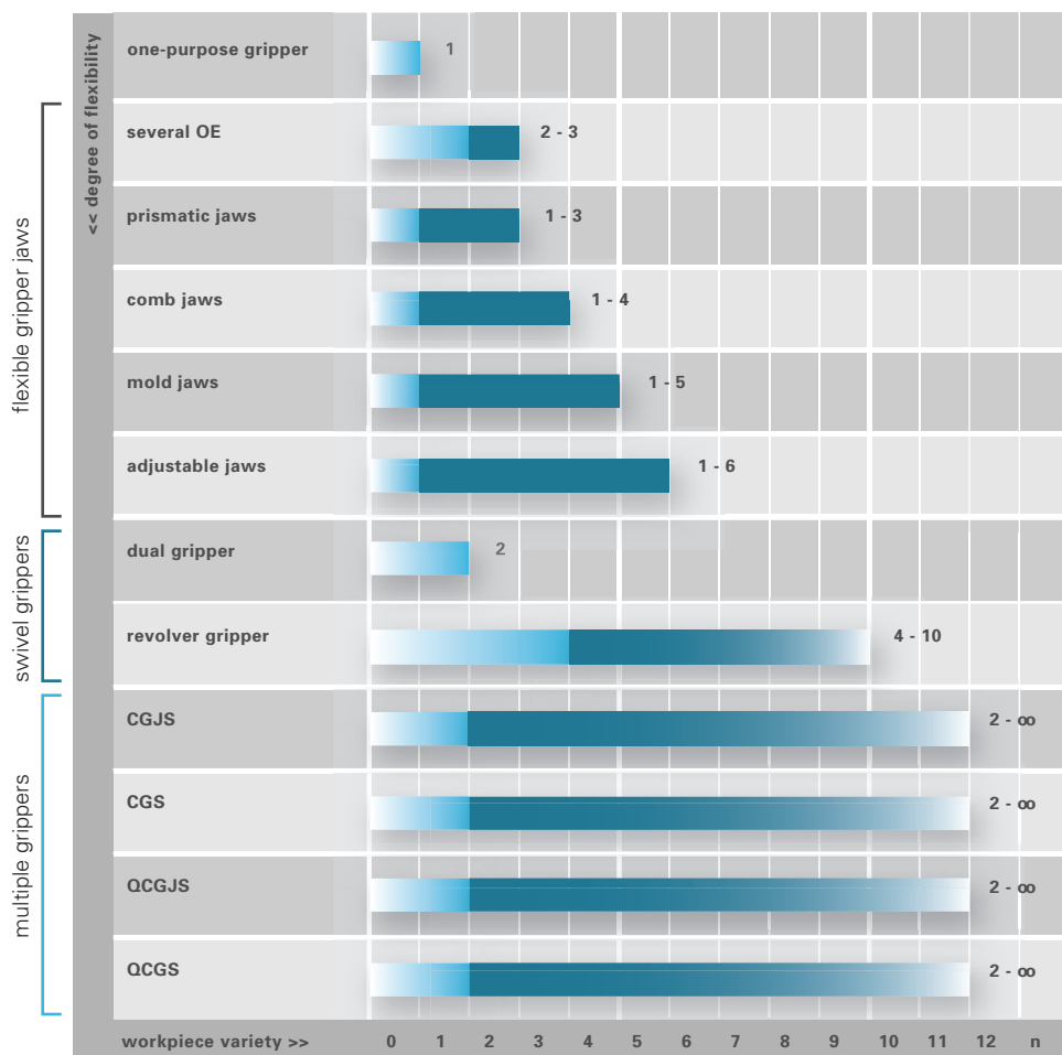
Figure 3.13 Flexible gripper systems coping with workpiece variety
