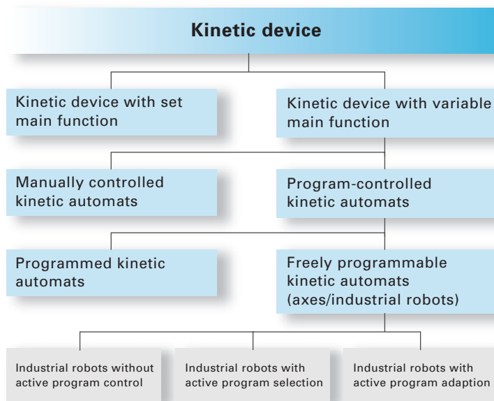
Figure 4.12 Kinetic device options (VDI 2860)
