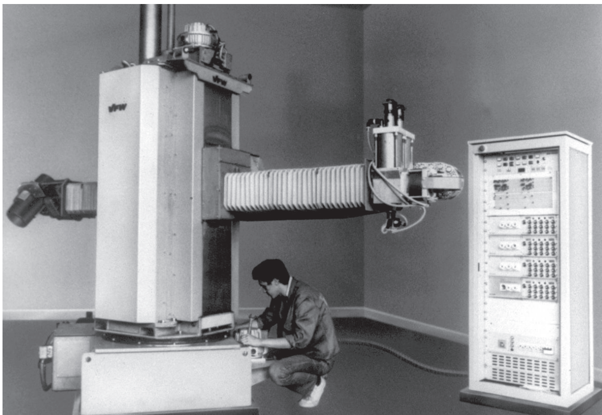
MBB-VFW robot with controller (source: Fraunhofer IPA)
