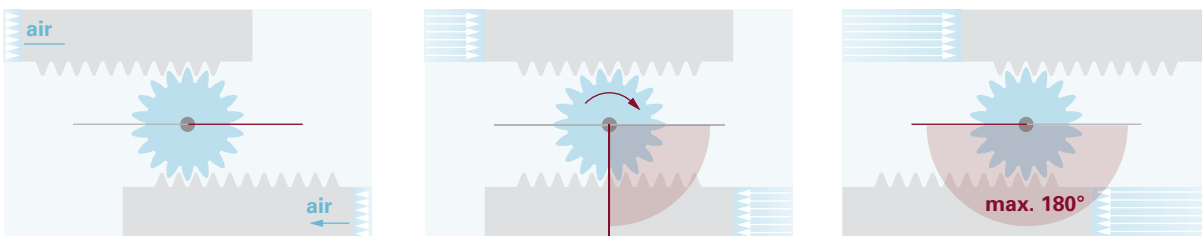
Figure 4.14 Swivel unit based on principle of pinion tooth rack
