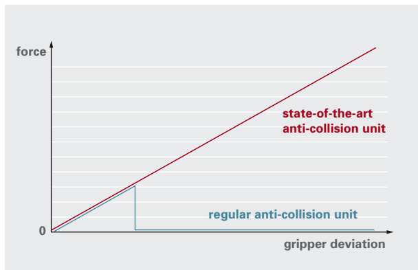
Figure 4.11 Force-deviation diagram for anti-collision units
