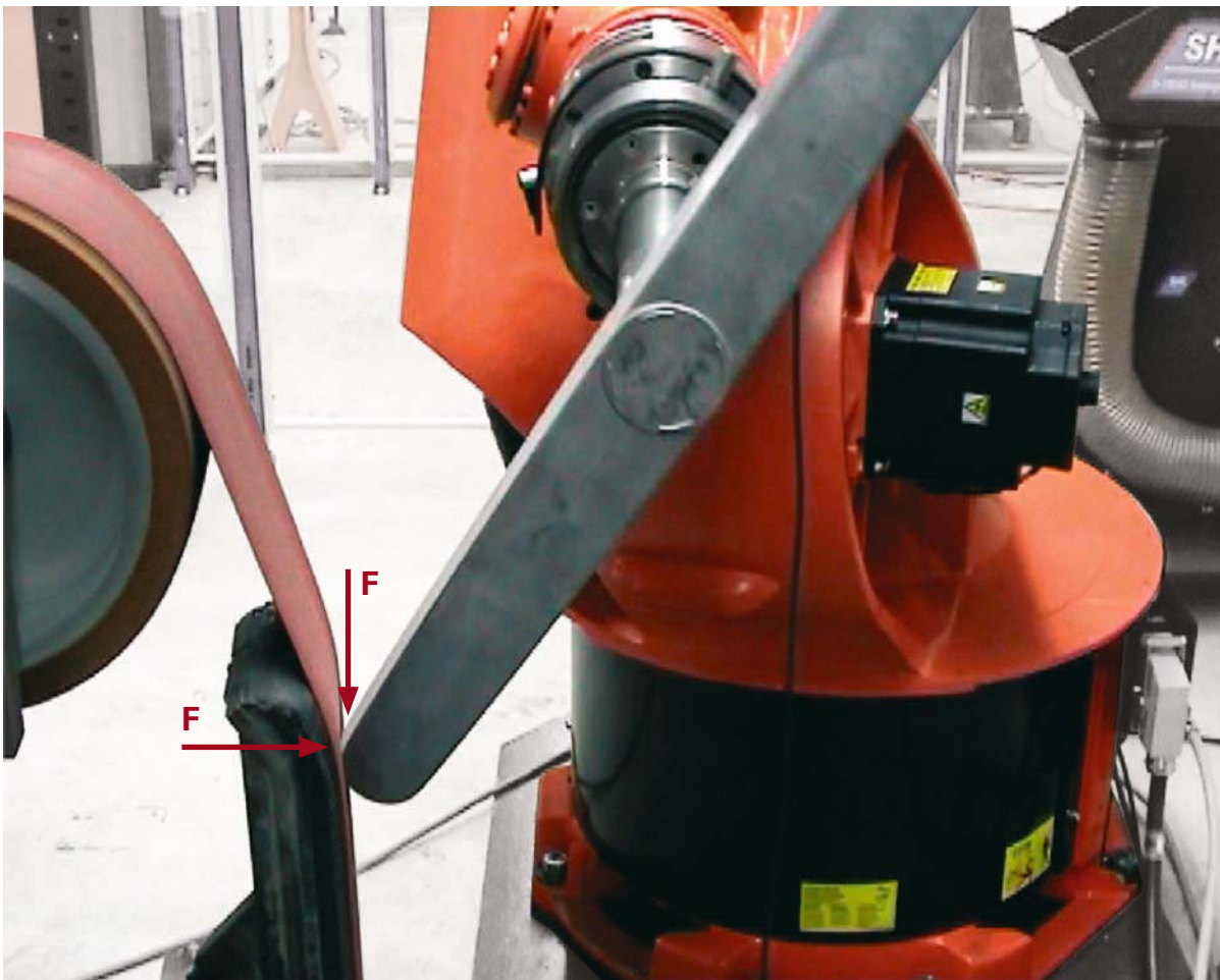
Force of process during workpiece polishing (source: ATI Theta Steifer KMS)
