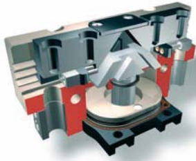
2-finger gripper
