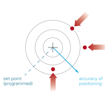
Figure 4.33 Deviations from the set point when approaching it from various directions (accuracy of positioning)
