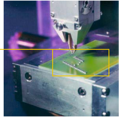
Place operation in the macro range (source: IPT)
