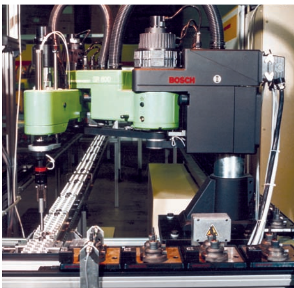
Left: BOSCH SCARA series SR800 at a double belt transfer system (source: Bosch Rexroth)
