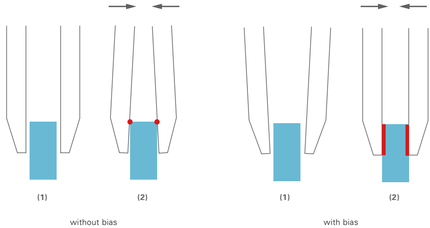
Figure 3.3 Avoiding point contact with the workpiece by gripper jaw bias
