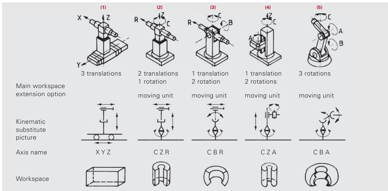
Figure 2.7 1983 regular kinematic types and their workspaces
