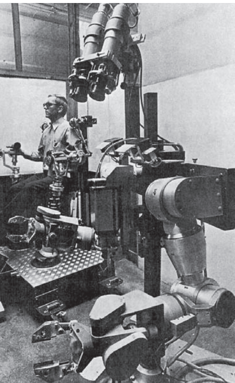
Syntelmann II Electric tele manipulator with 9 degrees of freedom per arm, position- and force-controlled, sensors for forces, sounds, temperatures (in front); operator with exo-skeleton transducer system, force feedback system, and stereo image transmission system (in the back). (Source: K. H. Dröge)
