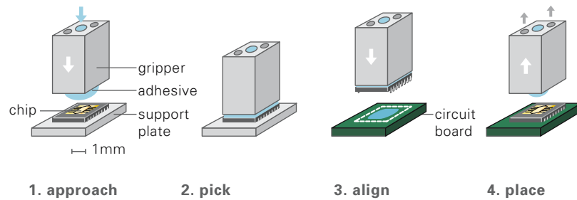
Figure 3.6 Adhesive gripping process (source: Bark)
