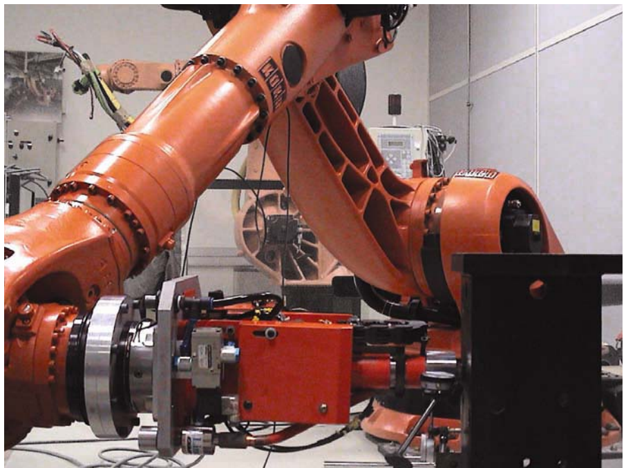
Robots with fixture for drilling (source: ATI Theta Steif, KMS)
