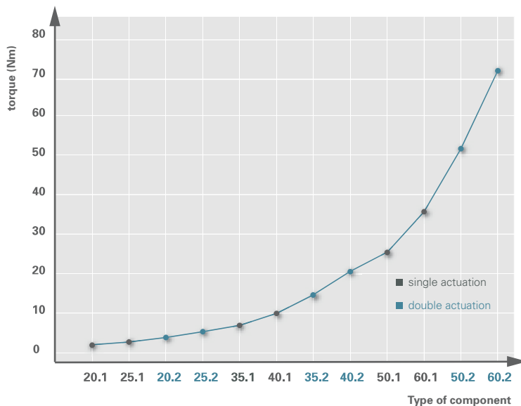
Figure 4.17 Graduation of torque for different swivel unit sizes
