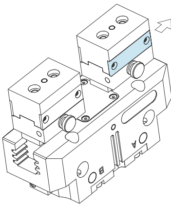
change unit for gripper fingers
