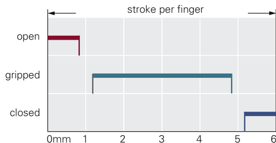
Figure 3.28 Pre-set areas where the proximity switch releases a signal
