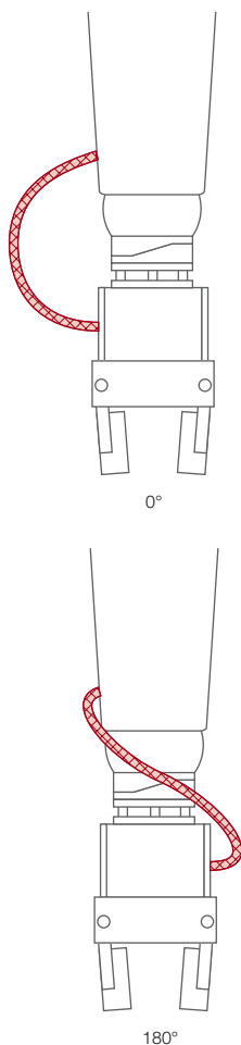
Figure 4.18 Rotation of the gripper, external guidance of tubes
