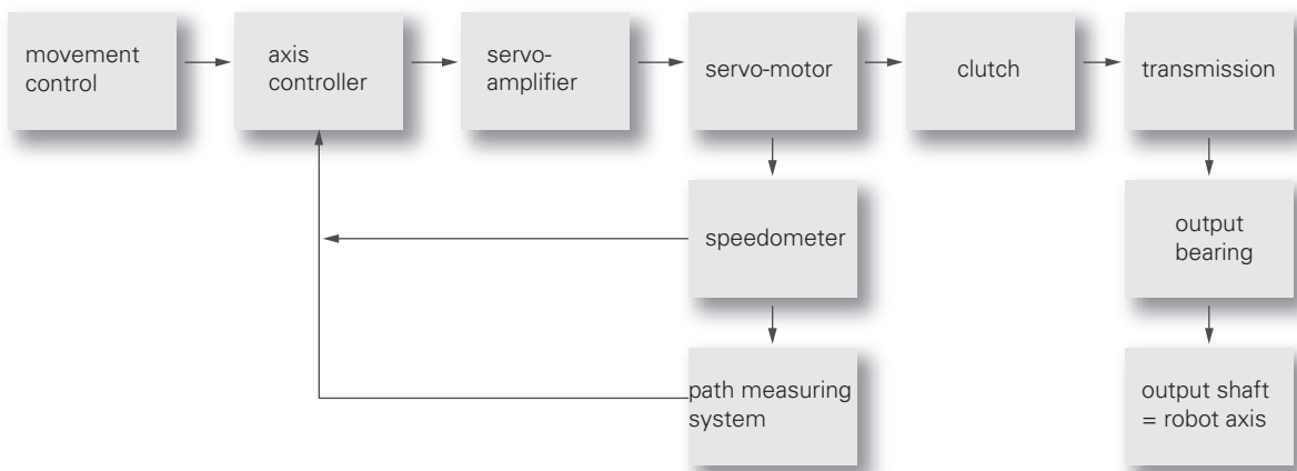
Figure 4.21 Components of a freely programmable axis
