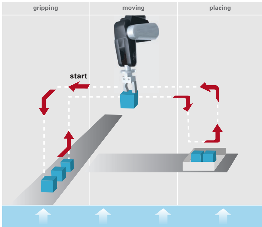
Figure 1.3 Phases of a handling process and its ambient conditions
