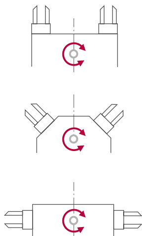
parallel, coniform and radial structure of revolver grippers
