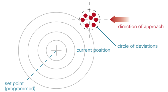
Figure 4.33 Deviations from the programmed set point when approaching from one direction (accuracy of repeatability)
