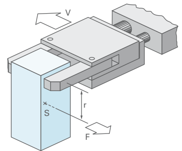
Figure 4.5 Displaced gripper fingers
