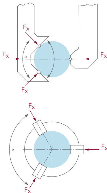
Figure 3.14 Gripping force is to be decomposed according to number of contact surfaces and number of fingers
