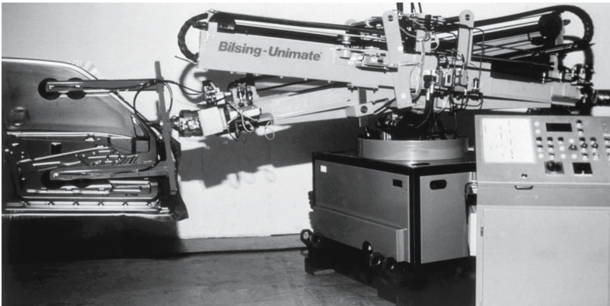
Bilsing Unimate robot for press handling (source: Fraunhofer IPA)
