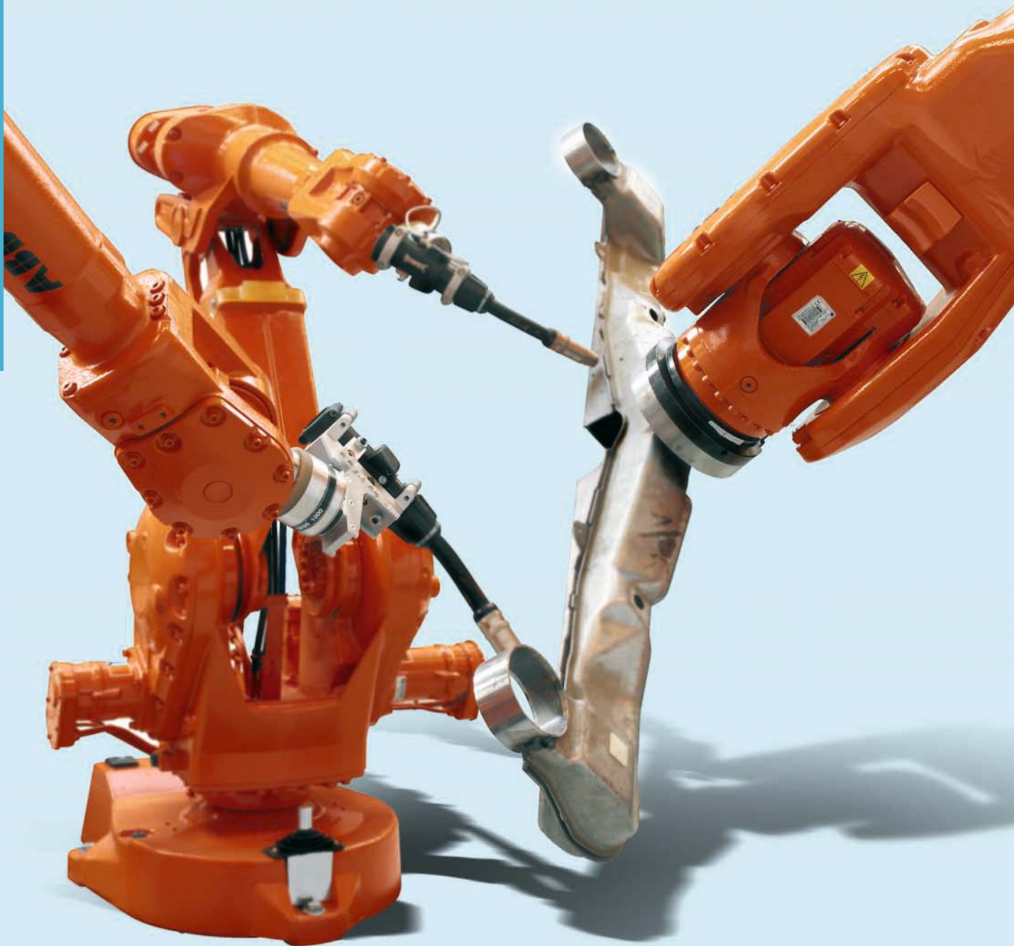
Flexible workpiece preparation for manufacturing car bodies with the help of synchronized robot movements
