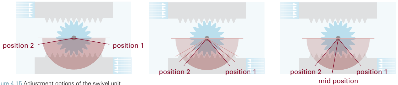
Figure 4.15 Adjustment options of the swivel unit
