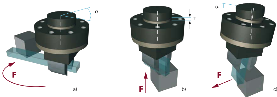
Figure 4.10 Examples of collisions with the respective directions of force and torque
