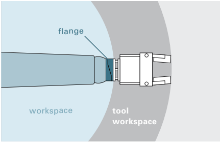
Figure 4.23 Restricted operational workspace and tool workspace
