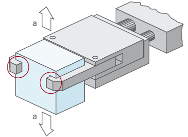
Figure 3.9 Form-fit gripping
