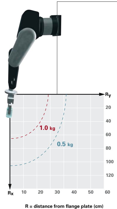
Figure 4.25 Example of a payload diagram for a robot with 1kg payload
