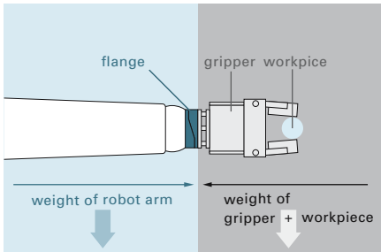
Figure 4.24 Stress on the kinetic device with gripper and workpiece combined
