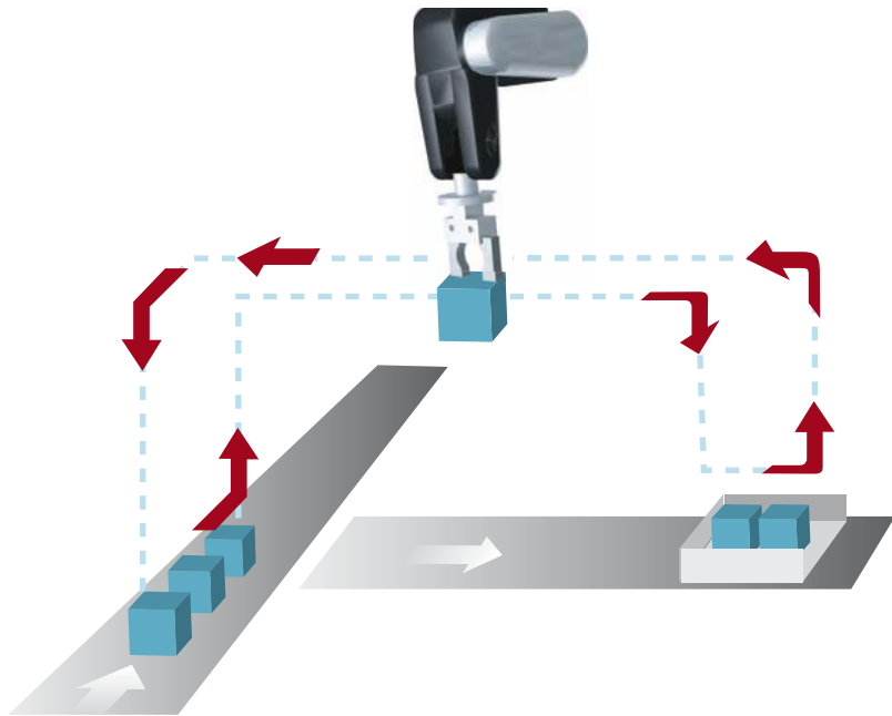
Figure 3.18 Direct linkage of workpiece input with workpiece output in a place position
