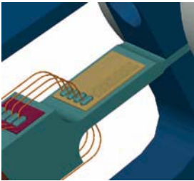
Evaluation unit with circuit board
