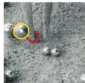
SEM image of glass spheres moved by electrostatic charge
