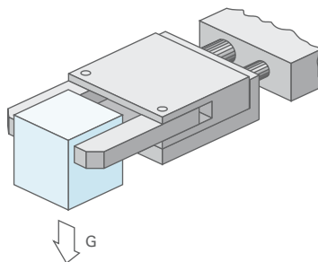
Figure 4.1 Static gripping: gripping force must compensate weight
