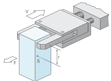
Figure 4.6 Slipping workpiece
