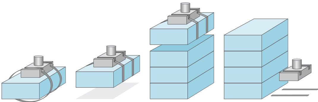
Figure 3.8 Baggage gripper – principle of function
