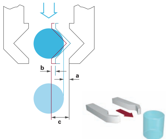
Figure 3.18 Radial grip
