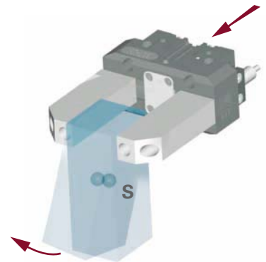
Figure 3.27 Braking movement of a robot with an unfavorable workpiece geometry within the gripper
