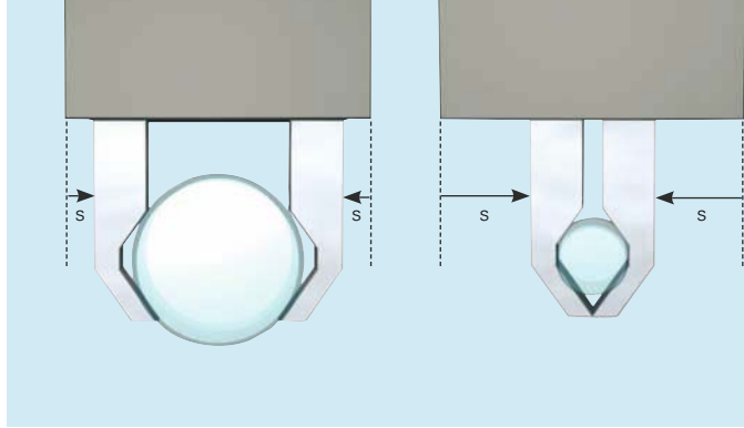
Picking up different material diameters with a prism illustrates the role of the finger stroke ( s ) for gripper flexibility
