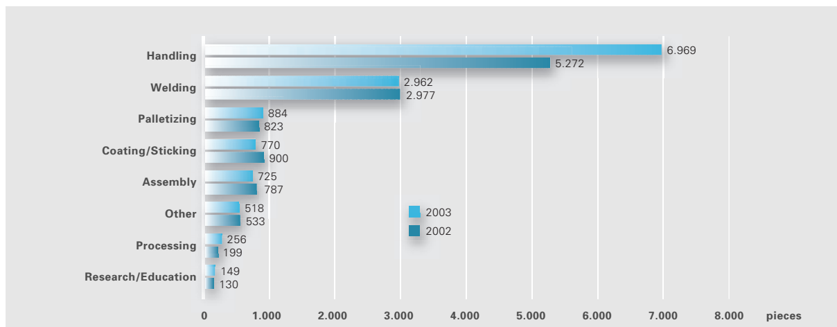
Figure 2.11 One- and two-axis moving modules – applications 2002 and 2003 (source: VDMA)
