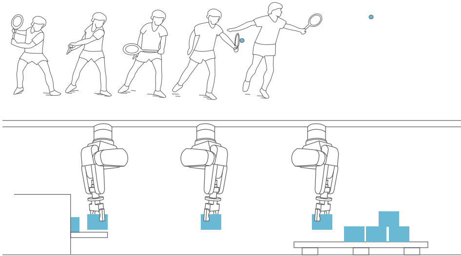
Figure 1.1 Motion sequence human/robot
