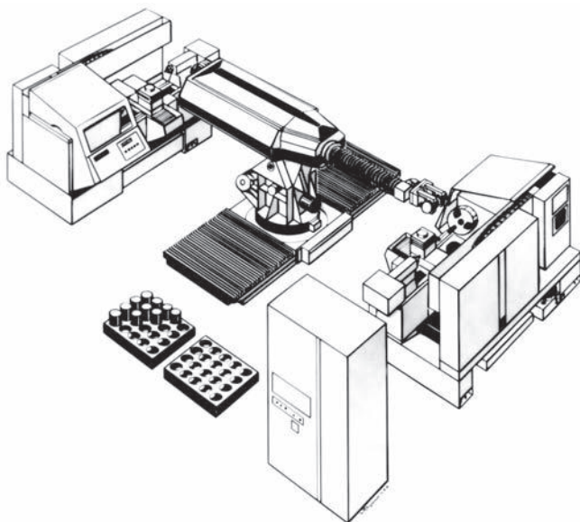
Plans for the use of a VW robot for feeding tooling machines (source: Fraunhofer IPA)
